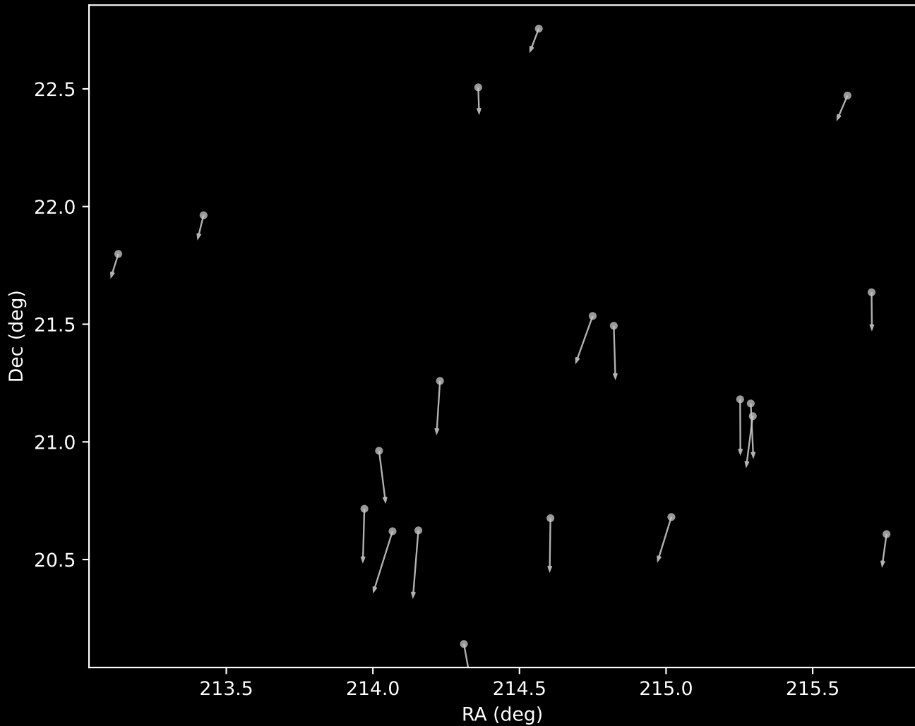
APOGEE DR17 Cluster 15 Proper Motion Vectors (n=20)
