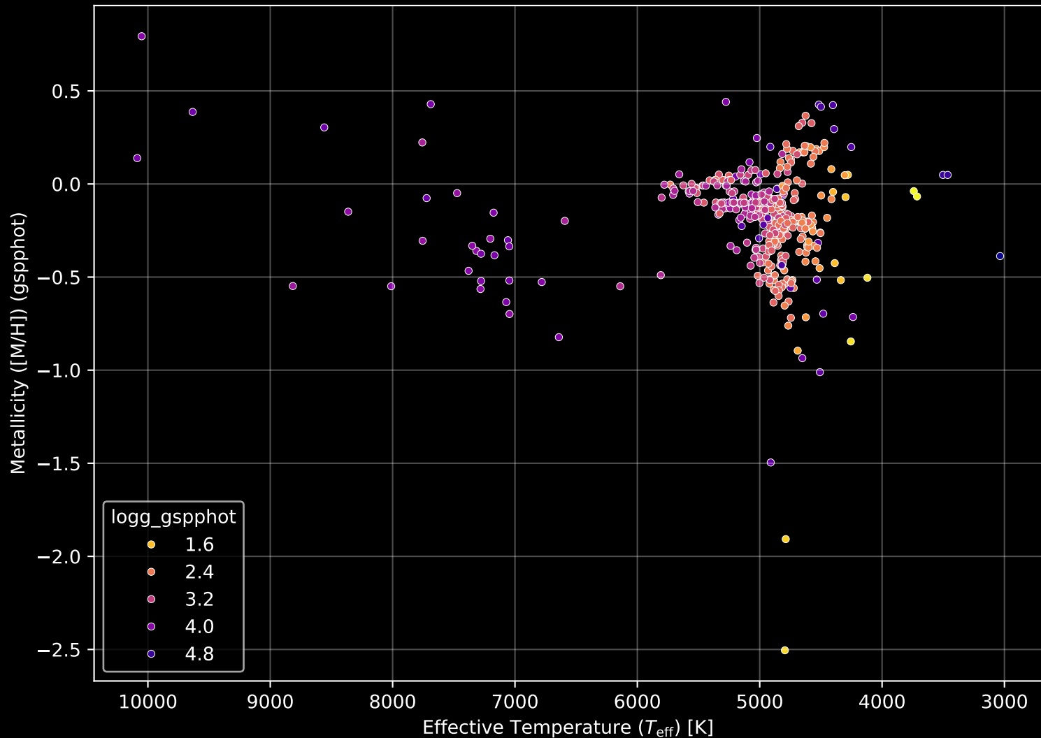
APOGEE DR17 Field: [N2420] Stellar Population Parameters (n= 471)
