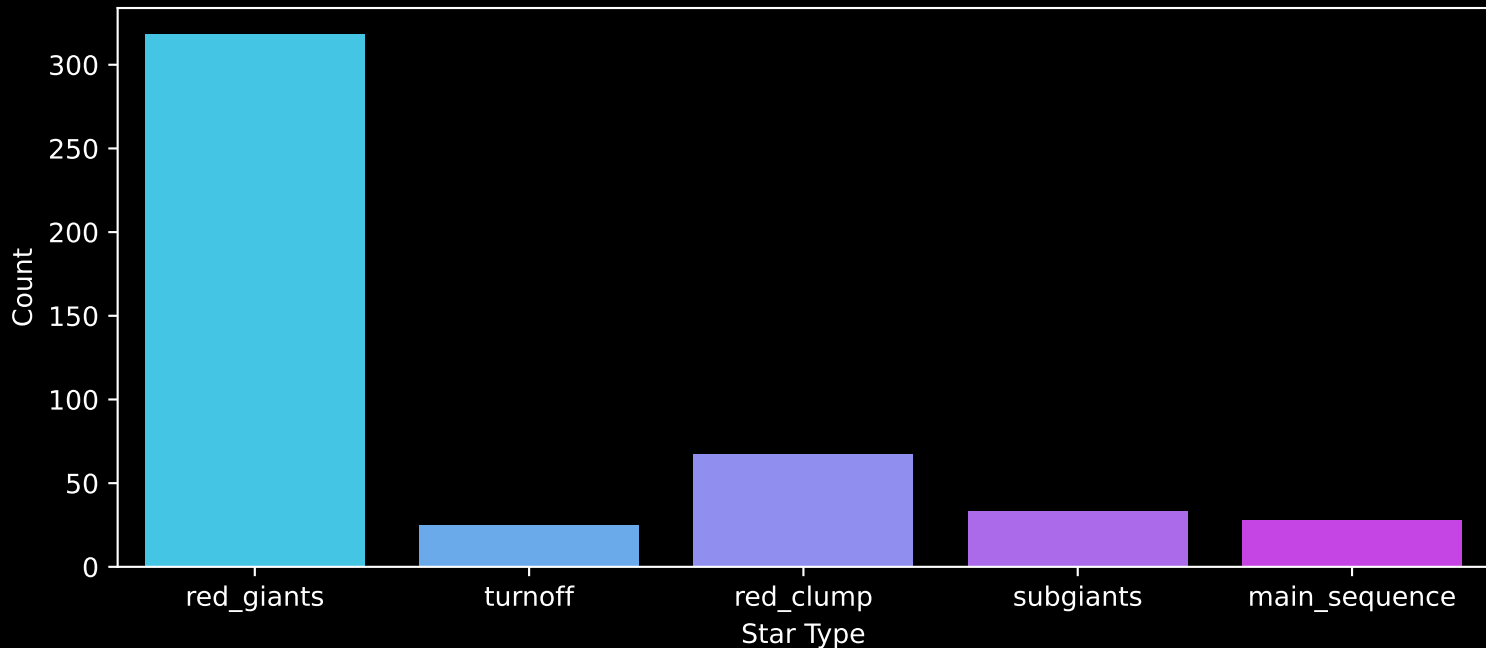
APOGEE DR17 Field: [N2420] Count plot of Star Type
