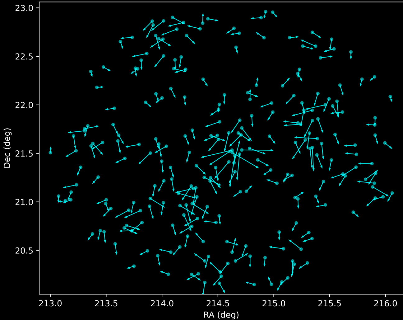
APOGEE DR17 Noise Stream Proper Motion Vectors (n=245)
