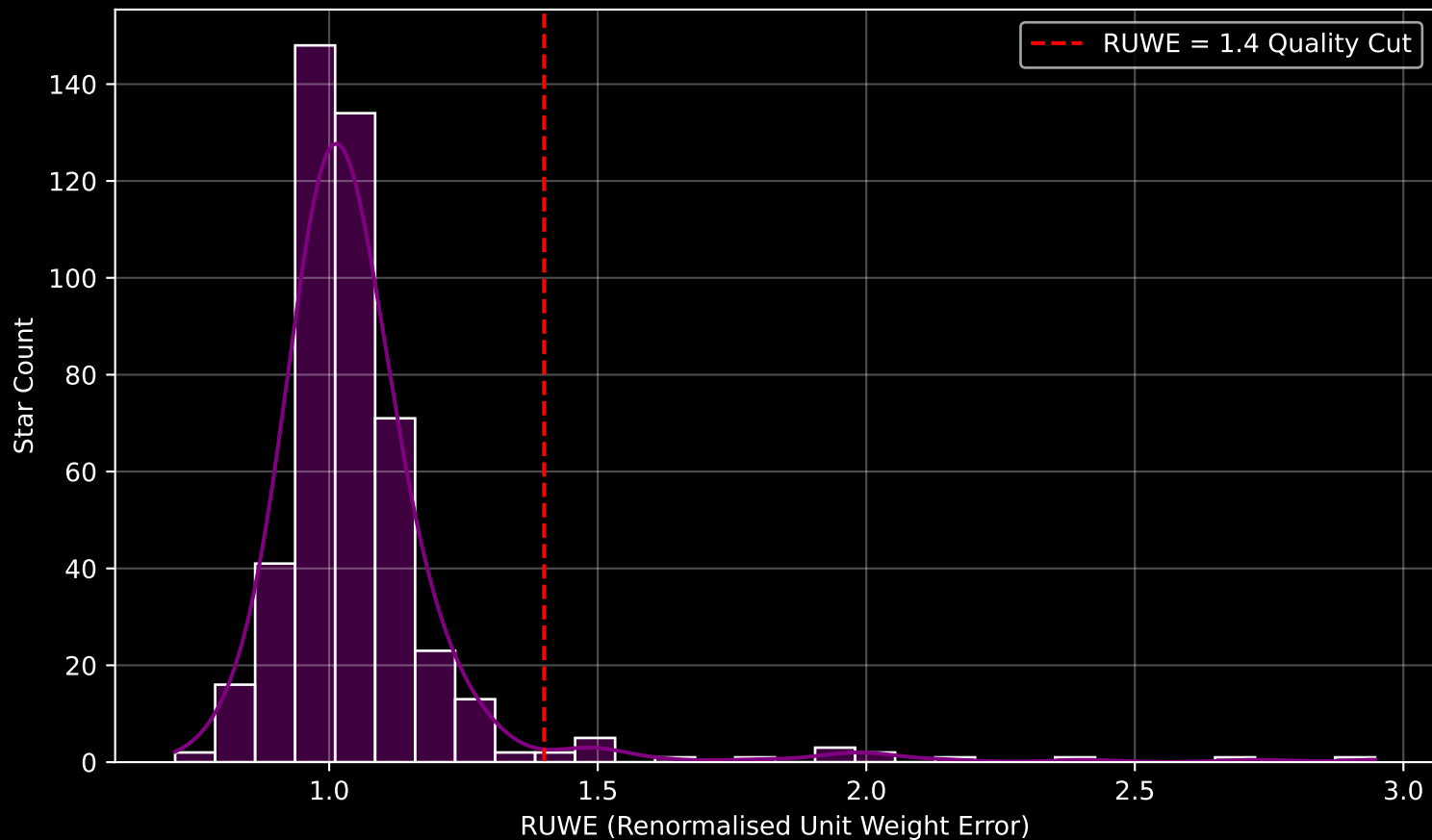
GAPOGEE DR17 Field [N2420] RUWE Distribution (n= 468)
