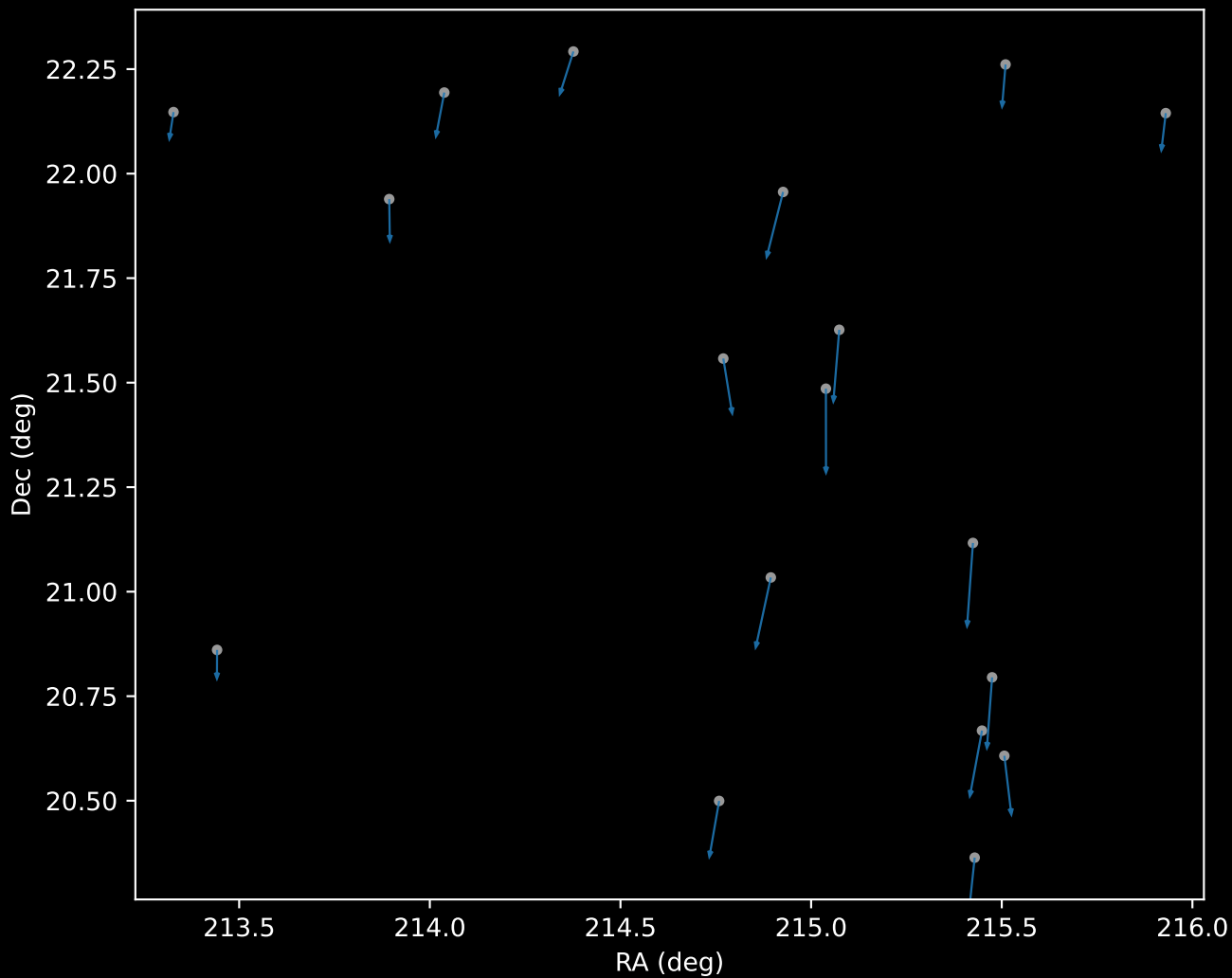
APOGEE DR17 Cluster 20 Proper Motion Vectors (n=18)
