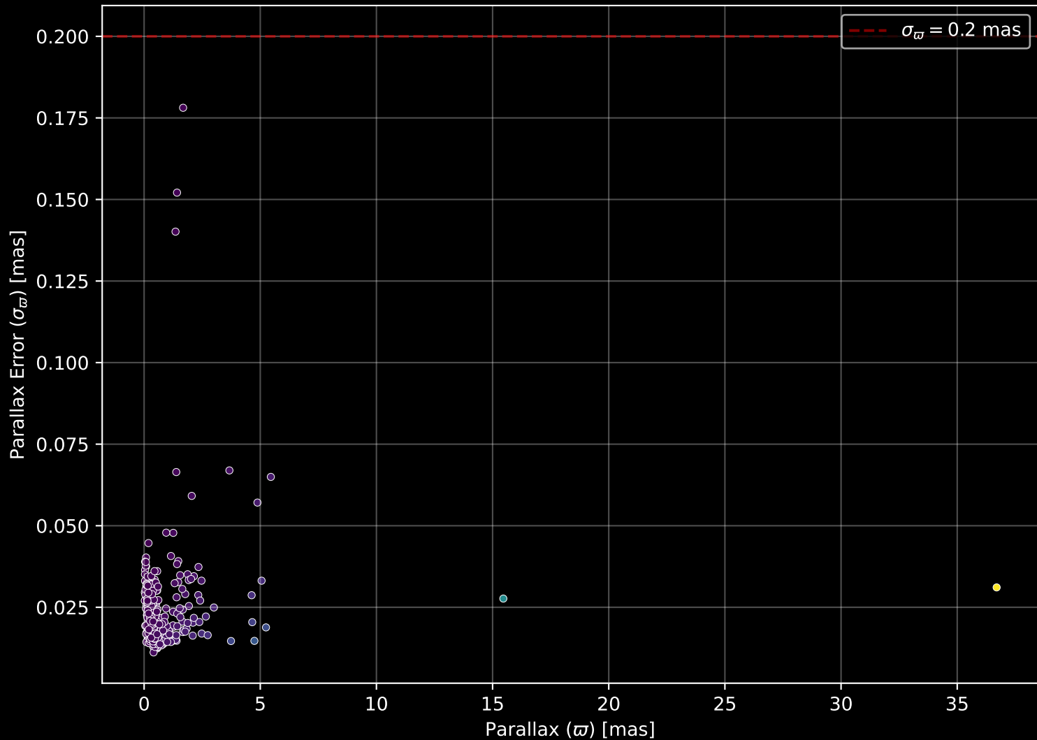
APOGEE DR17 Field: [N2420] Parallax Quality (n= 471)
