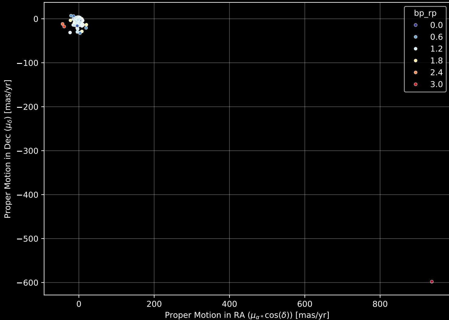
APOGEE DR17 Field: [N2420] Proper Motion Diagram (n= 471)
