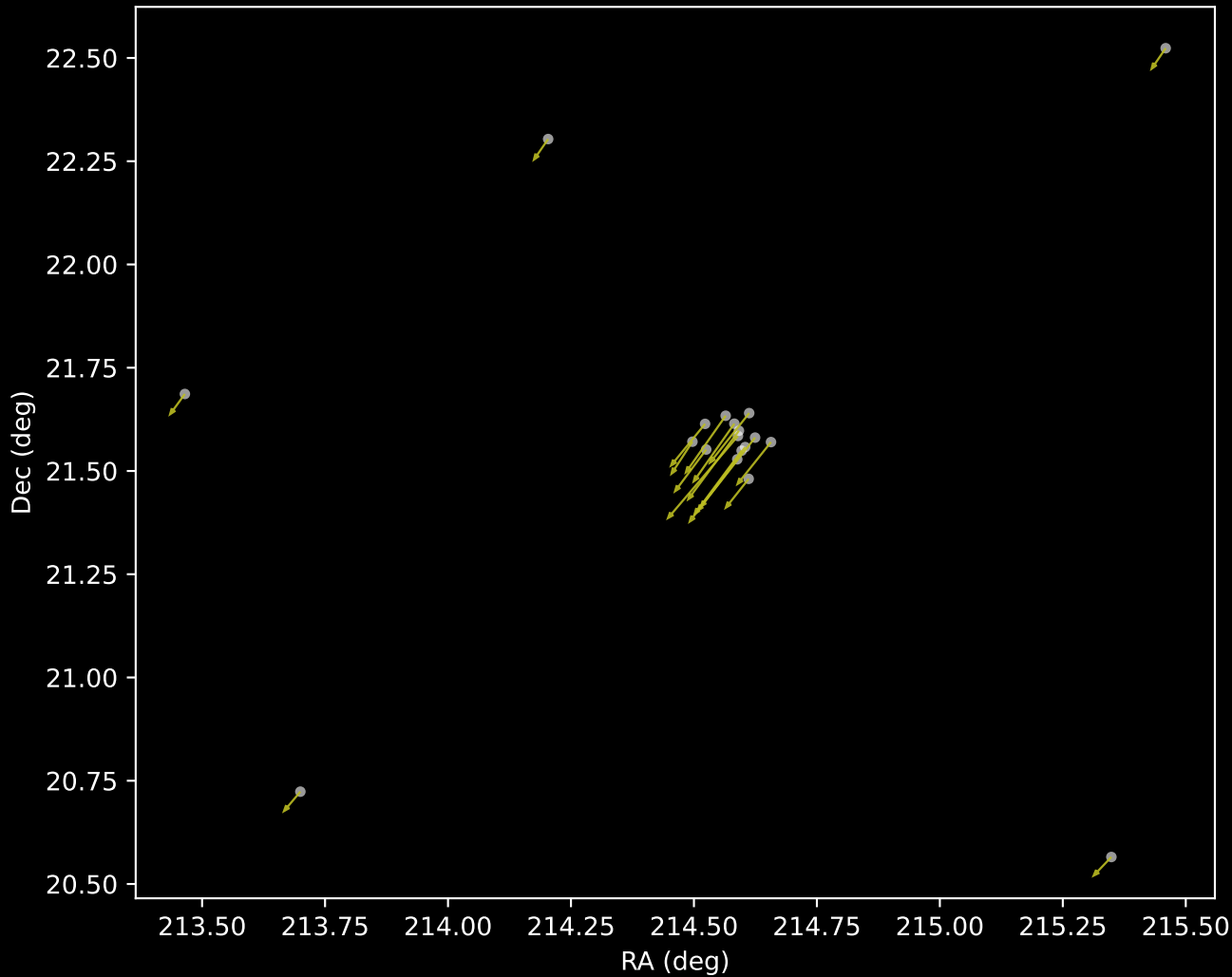
APOGEE DR17 Cluster 16 Proper Motion Vectors (n=19)
