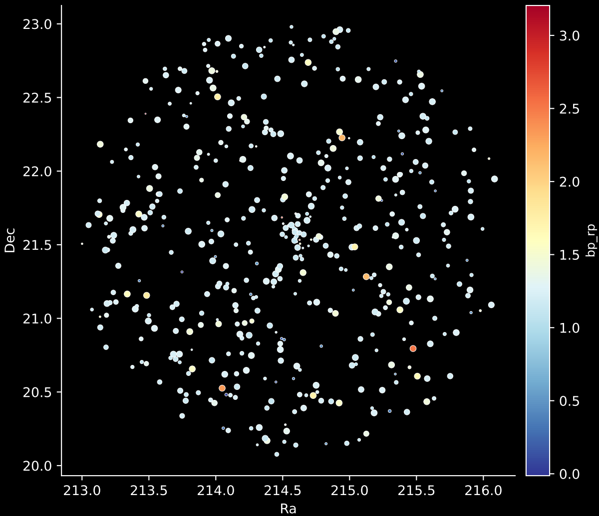
APOGEE DR17 Field: [N2420] Stars: 471
