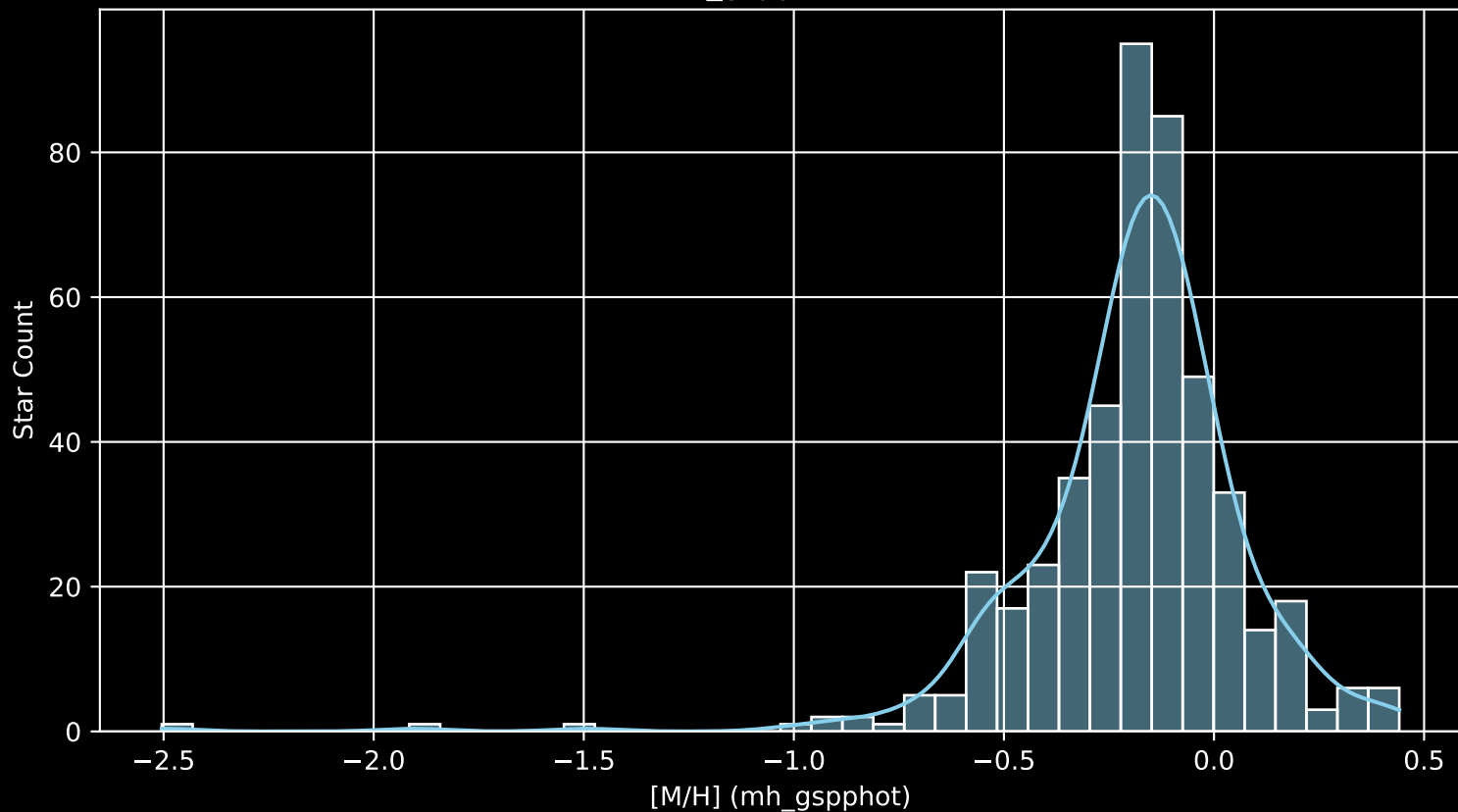
APOGEE DR17 Field: [N2420 [M/H] (mh_gspphot) (n= 470)
